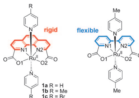
Figure 1. Molecular structures of 1a–c and [\text{Ru}^{\text{II}}(\text{bda})(\text{pic})_2] ( 2 ).
